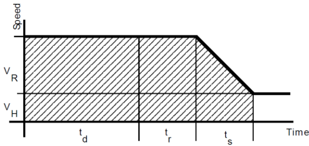
Figure 3. SSM Stopping Diagram [10].
